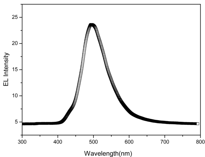
FIGURE 3 EL spectrum of ITO/PEDOT:PSS(50 nm)/POTOSF(70 nm)/LiF(1 nm)/Al(200 nm) device at 20 mA/cm 2 .
