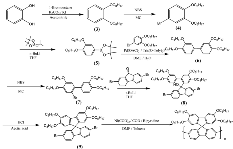
SCHEME 2 Synthetic route of PTOSF.
