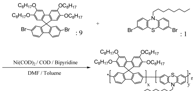
SCHEME 3 Synthetic route of POTOSF.
