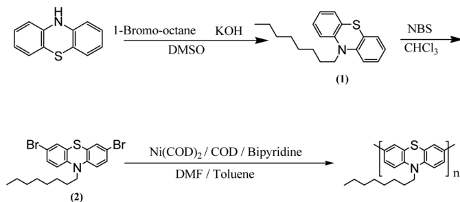
SCHEME 1 Synthetic route of POP.
